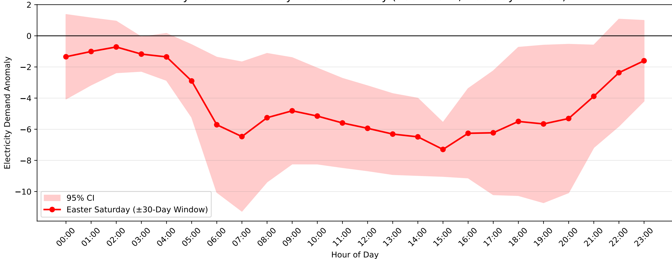
Hornsby Demand Anomaly: Easter Saturday (2004-2017, \pm 30 -Day Window)
